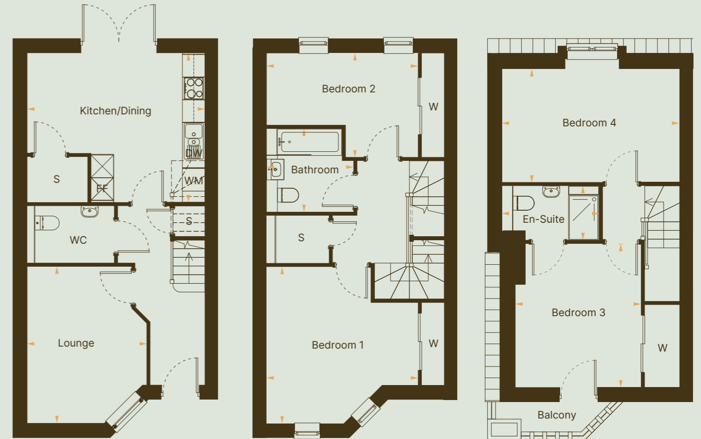
GROUND FLOOR
